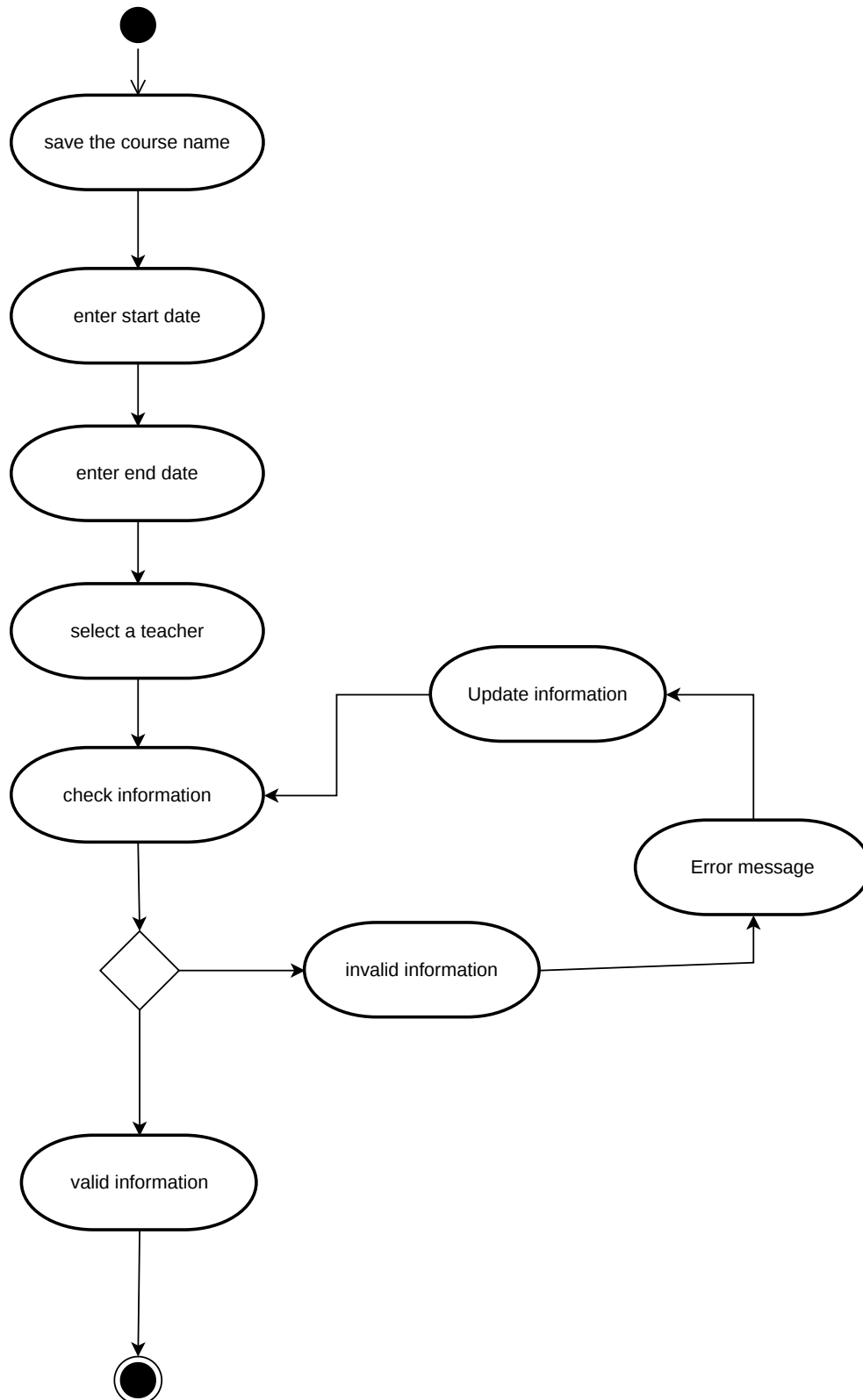
Activity Diagram : Manage a course
